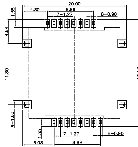
RECOMMENDED PC BOARD LAYOUT TOLFRANCF: +0.05[TOP VIFW]
